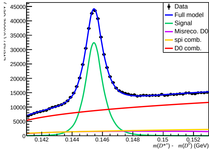
Failed ( 200 < n\text{Tracks} < 600 , 1.7 < \eta < 3.6 , 3000 < p < 6000 )
