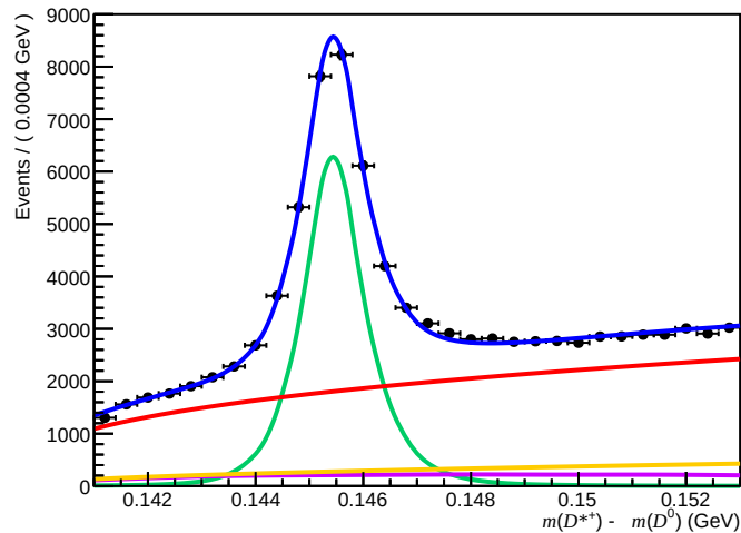
Passed ( 200 < n\text{Tracks} < 600 , 1.7 < \eta < 3.6 , 3000 < p < 6000 )
