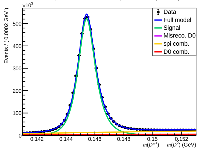
Failed ( 200 < nTracks < 600 , 1.7 < \eta < 3.6 , 27000 < p < 60000 )
