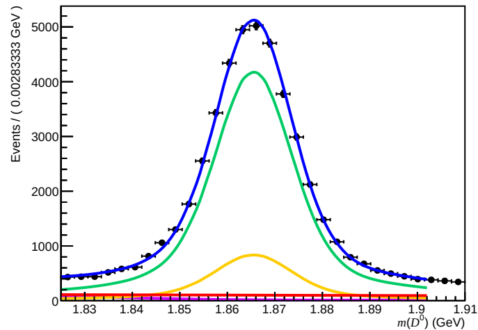
Failed ( 200 < nTracks < 600 , 1.7 < \eta < 3.6 , 27000 < p < 60000 )
