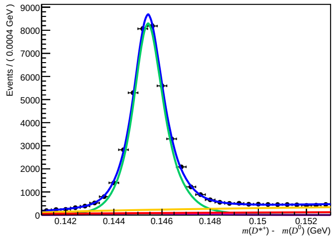
Failed ( 200 < nTracks < 600 , 1.7 < \eta < 3.6 , 27000 < p < 60000 )
