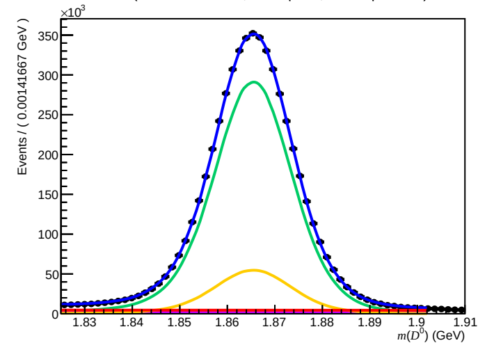
Failed ( 200 < nTracks < 600 , 1.7 < \eta < 3.6 , 27000 < p < 60000 )
