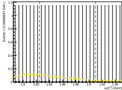
Passed ( 200 < nTracks < 600 , 3.6 < \eta < 5.0 , 6000 < p < 10000 )
