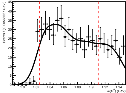
Failed ( 200 < nTracks < 600 , 3.6 < \eta < 5.0 , 6000 < p < 10000 )
