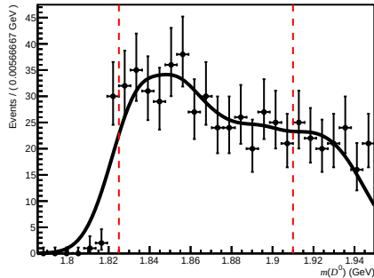
Total ( 200 < nTracks < 600 , 3.6 < \eta < 5.0 , 6000 < p < 10000 )
