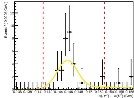
Total ( 200 < nTracks < 600 , 3.6 < \eta < 5.0 , 10000 < p < 15600 )
