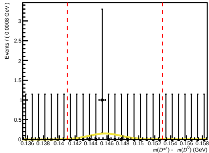
Passed ( 200 < nTracks < 600 , 3.6 < \eta < 5.0 , 10000 < p < 15600 )
