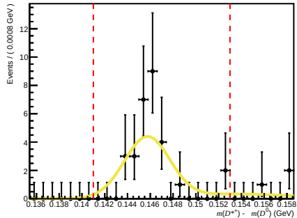
Failed ( 200 < nTracks < 600 , 3.6 < \eta < 5.0 , 10000 < p < 15600 )
