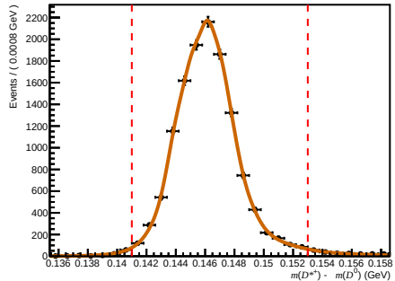
Total ( 200 < nTracks < 600 , 3.6 < \eta < 5.0 , 15600 < p < 27000 )
