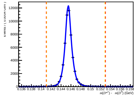
Failed DiF ( 0 < n_{\text{Tracks}} < 200 , 1.7 < \eta < 3.6 , 15600 < p < 27000 )
