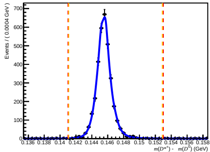
Passed DiF (after RICH1) ( 0 < n_{\text{Tracks}} < 200 , 1.7 < \eta < 3.6 , 15600 < p < 27000 )
