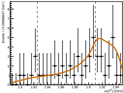
Passed ( 0 < n\text{Tracks} < 200 , 1.7 < \eta < 3.6 , 27000 < p < 60000 )
