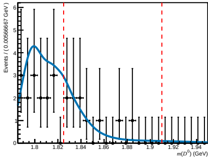
Passed ( 200 < nTracks < 600 , 3.6 < \eta < 5.0 , 27000 < p < 60000 )
