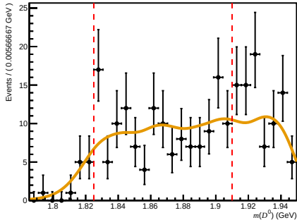
Passed ( 0 < n_{\text{Tracks}} < 200 , 1.7 < \eta < 3.6 , 3000 < p < 6000 )
