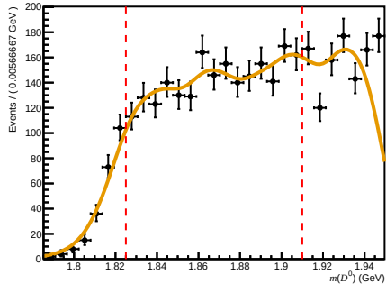
Failed ( 0 < n_{\text{Tracks}} < 200 , 1.7 < \eta < 3.6 , 3000 < p < 6000 )
