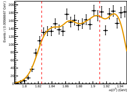
Total ( 0 < n_{\text{Tracks}} < 200 , 1.7 < \eta < 3.6 , 3000 < p < 6000 )
