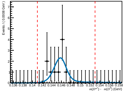
Passed ( 0 < nTracks < 200 , 1.7 < \eta < 3.6 , 6000 < p < 10000 )
