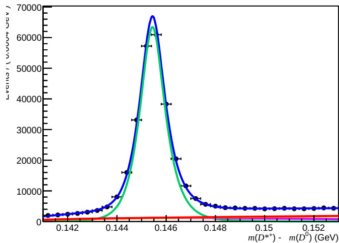
Failed ( 0 < nTracks < 200 , 1.7 < \eta < 3.6 , 6000 < p < 10000 )
