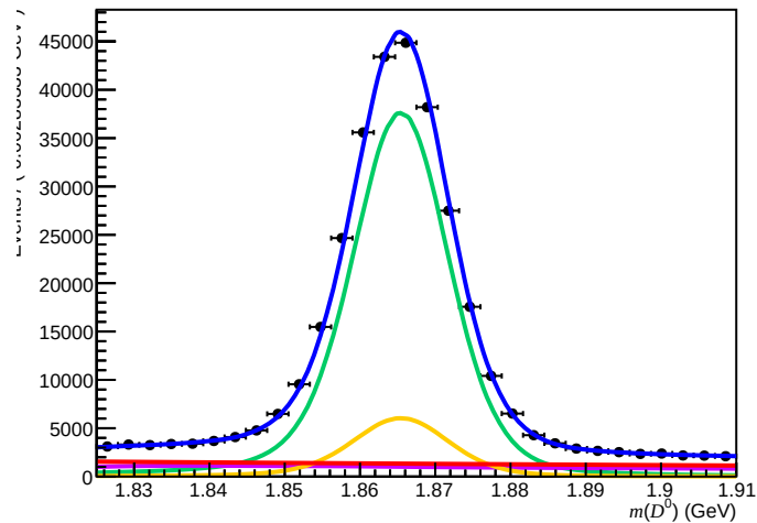
Failed ( 0 < nTracks < 200 , 1.7 < \eta < 3.6 , 6000 < p < 10000 )
