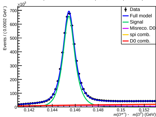
Failed ( 0 < nTracks < 200 , 1.7 < \eta < 3.6 , 6000 < p < 10000 )
