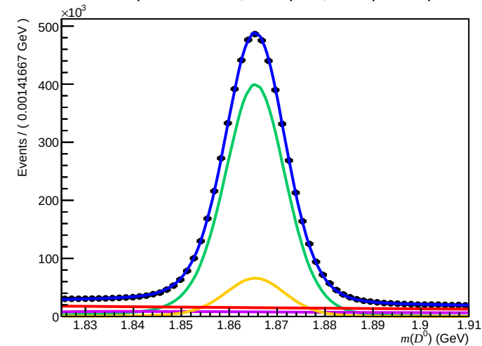
Failed ( 0 < nTracks < 200 , 1.7 < \eta < 3.6 , 6000 < p < 10000 )
