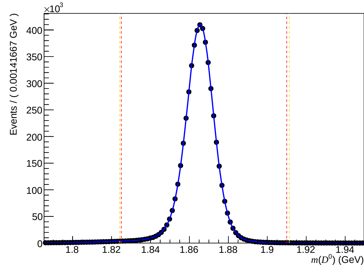
Failed non-DiF ( 0 < nTracks < 200 , 1.7 < \eta < 3.6 , 10000 < p < 15600 )
