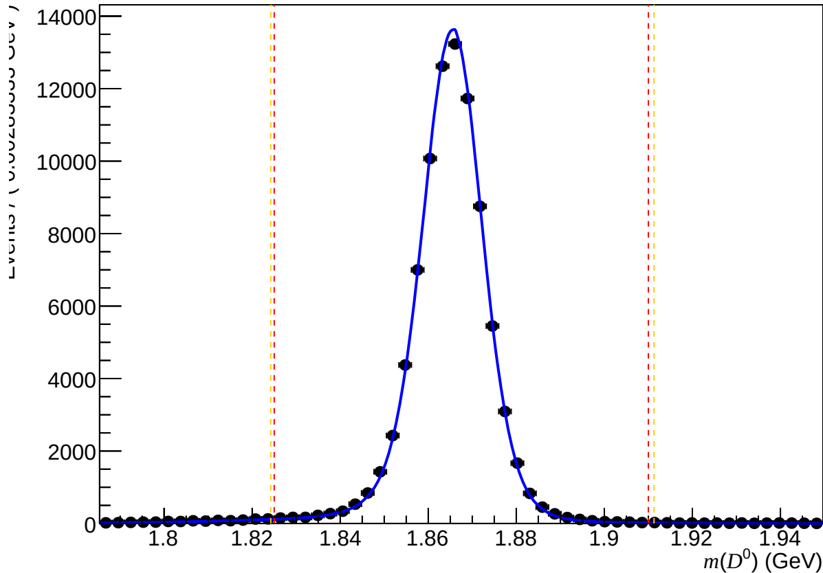
Passed non-DiF ( 0 < nTracks < 200 , 1.7 < \eta < 3.6 , 10000 < p < 15600 )
