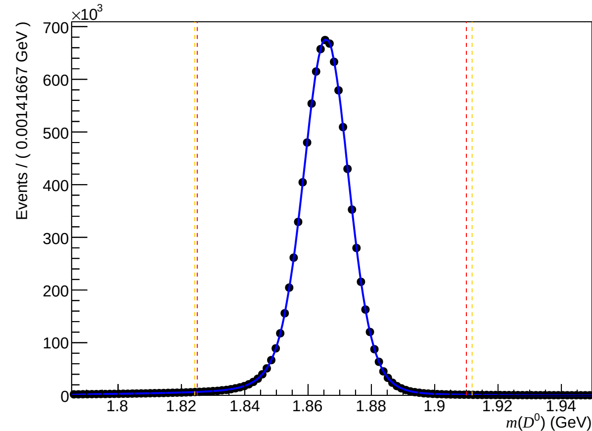
Failed non-DiF ( 0 < nTracks < 200 , 1.7 < \eta < 3.6 , 15600 < p < 27000 )
