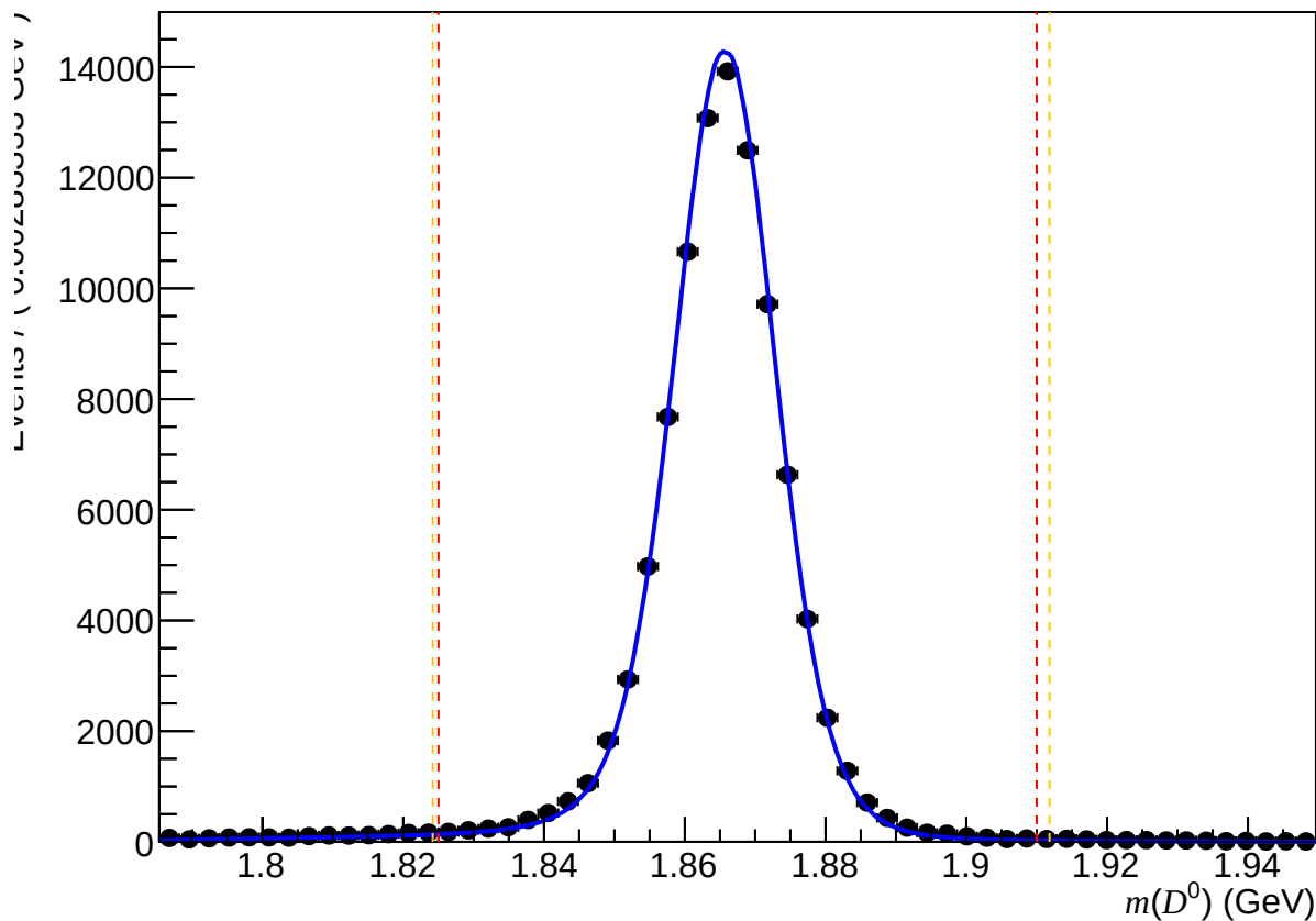
Passed non-DiF ( 0 < nTracks < 200 , 1.7 < \eta < 3.6 , 15600 < p < 27000 )
