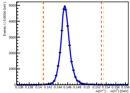
Passed DiF (after RICH1) ( 0 < n_{\text{Tracks}} < 200 , 1.7 < \eta < 3.6 , 27000 < p < 60000 )
