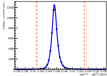
Failed DiF ( 0 < n_{\text{Tracks}} < 200 , 1.7 < \eta < 3.6 , 27000 < p < 60000 )
