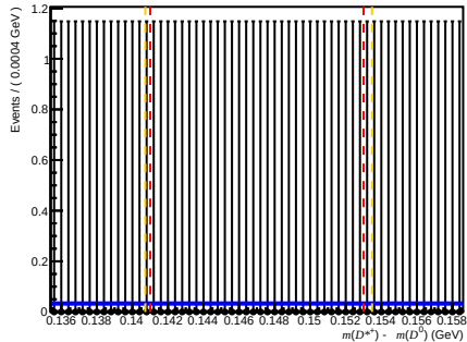
Passed DiF (before RICH1) ( 0 < n_{\text{Tracks}} < 200 , 1.7 < \eta < 3.6 , 27000 < p < 60000 )
