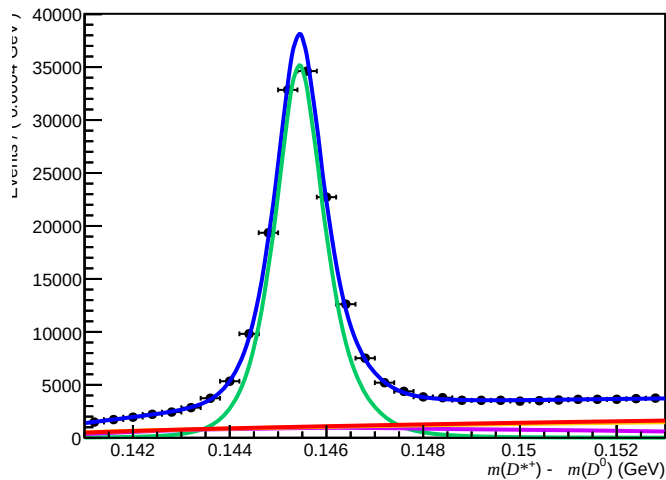
Passed ( 200 < n\text{Tracks} < 600 , 1.7 < \eta < 3.6 , 6000 < p < 10000 )
