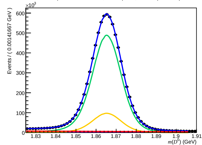
Failed (200 < nTracks < 600, 1.7 < \eta < 3.6, 15600 < p < 27000)
