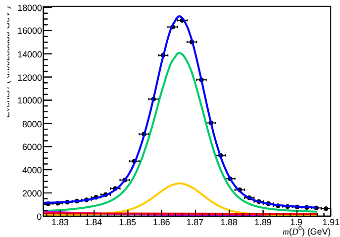
Passed (200 < nTracks < 600, 1.7 < \eta < 3.6, 15600 < p < 27000)
