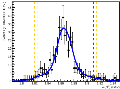
Passed DIF (after RICH1) ( 200 < n_{\text{Tracks}} < 600 , 3.6 < \eta < 5.0 , 6000 < p < 10000 )
