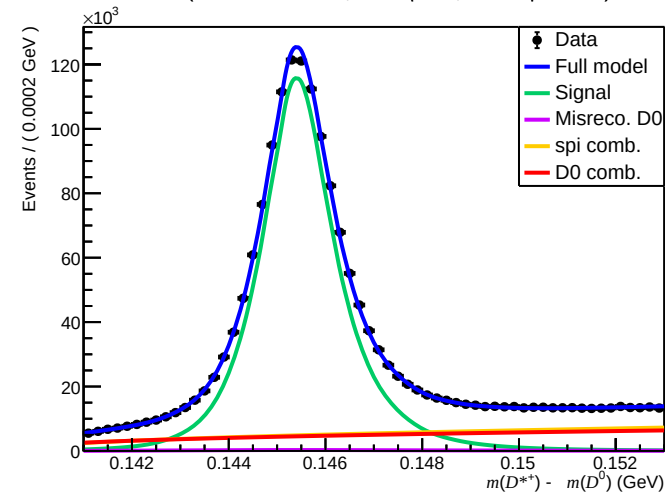
Failed (200 < nTracks < 600, 3.6 < \eta < 5.0, 15600 < p < 27000)
