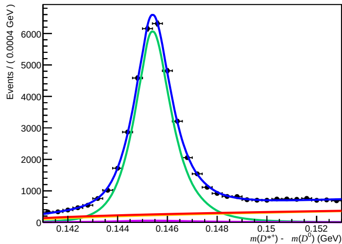
Failed (200 < nTracks < 600, 3.6 < \eta < 5.0, 15600 < p < 27000)
