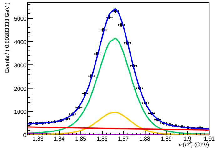
Failed (200 < nTracks < 600, 3.6 < \eta < 5.0, 15600 < p < 27000)
