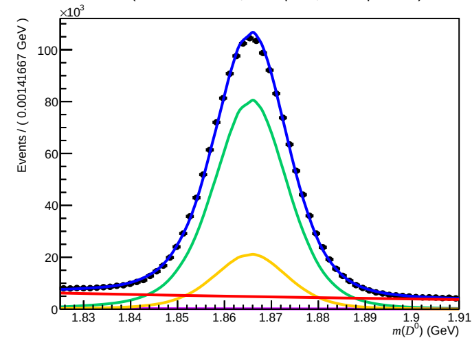
Failed (200 < nTracks < 600, 3.6 < \eta < 5.0, 15600 < p < 27000)
