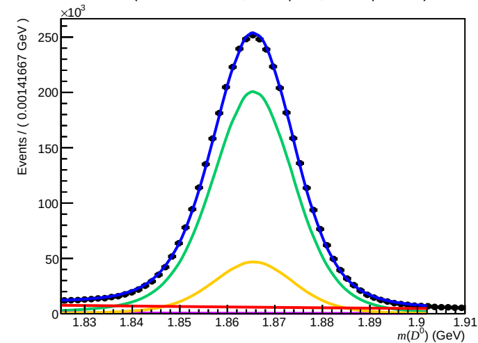
Failed ( 200 < n\text{Tracks} < 600 , 3.6 < \eta < 5.0 , 27000 < p < 60000 )
