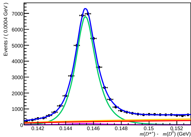
Failed ( 200 < n\text{Tracks} < 600 , 3.6 < \eta < 5.0 , 27000 < p < 60000 )
