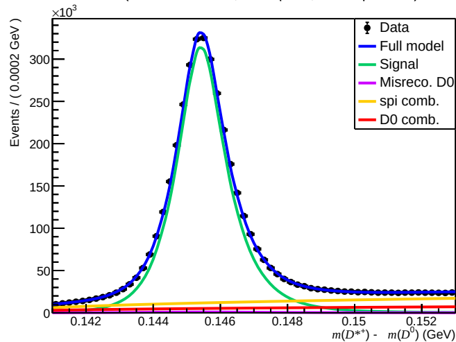
Failed ( 200 < n\text{Tracks} < 600 , 3.6 < \eta < 5.0 , 27000 < p < 60000 )
