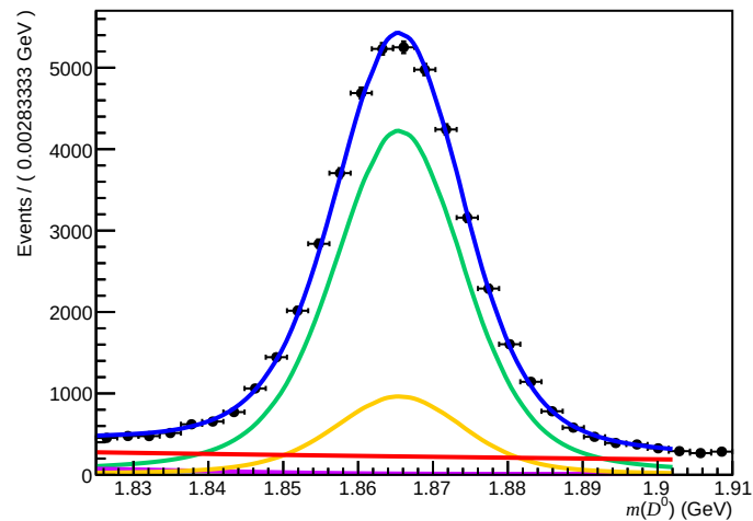
Failed ( 200 < n\text{Tracks} < 600 , 3.6 < \eta < 5.0 , 27000 < p < 60000 )
