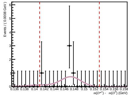
Total ( 0 < nTracks < 200 , 1.7 < \eta < 3.6 , 6000 < p < 10000 )
