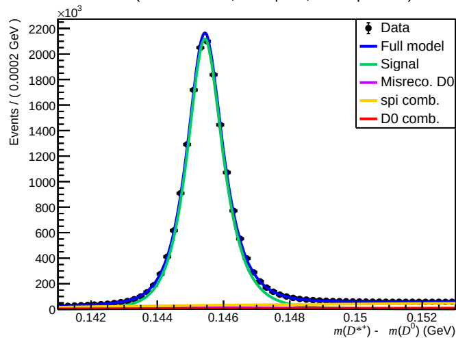
Failed ( 0 < n_{\text{Tracks}} < 200 , 1.7 < \eta < 3.6 , 15600 < p < 27000 )
