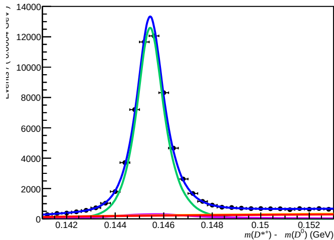
Passed ( 0 < n_{\text{Tracks}} < 200 , 1.7 < \eta < 3.6 , 15600 < p < 27000 )
