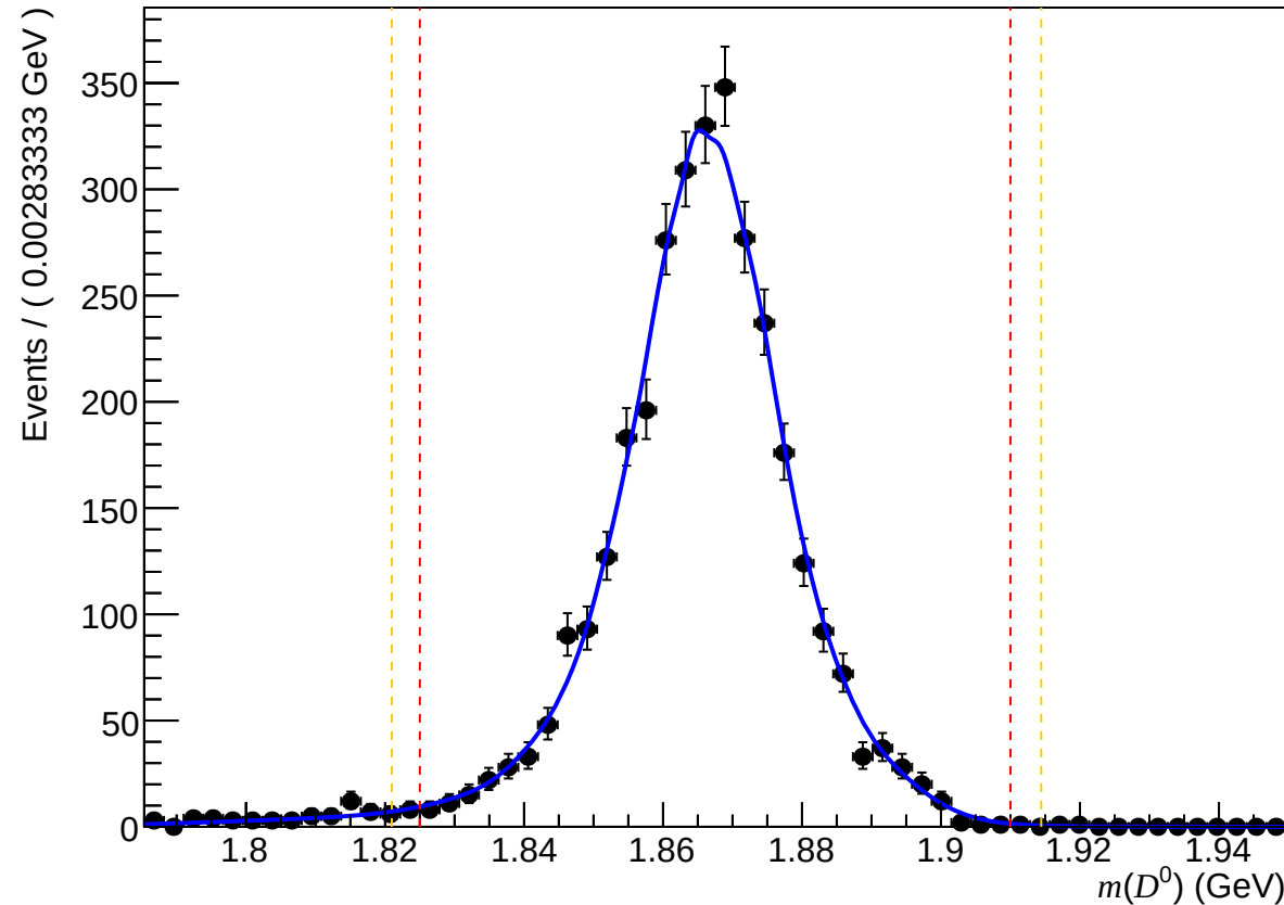
Passed non-DiF ( 0 < nTracks < 200 , 3.6 < \eta < 5.0 , 3000 < p < 6000 )
