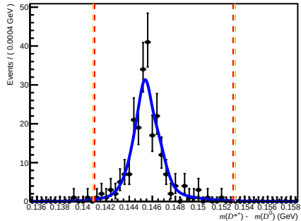
Passed DiF (after RICH1) ( 0 < n_{\text{Tracks}} < 200 , 3.6 < \eta < 5.0 , 3000 < p < 6000 )
