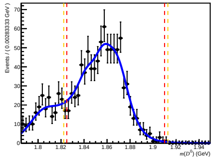
Passed DiF (after RICH1) ( 0 < n_{\text{Tracks}} < 200 , 3.6 < \eta < 5.0 , 10000 < p < 15600 )
