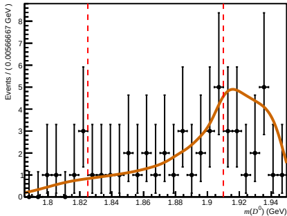
Passed ( 0 < n_{\text{Tracks}} < 200 , 3.6 < \eta < 5.0 , 27000 < p < 60000 )
