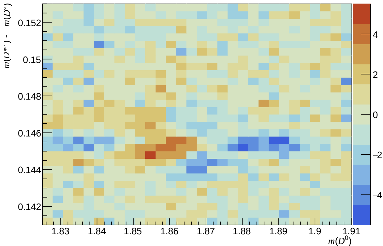
Passed ( 200 < nTracks < 600 , 1.7 < \eta < 3.6 , 6000 < p < 10000 )
