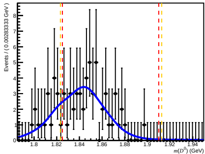
Passed DiF (after RICH1) ( 200 < nTracks < 600 , 1.7 < \eta < 3.6 , 60000 < p < 100000 )
