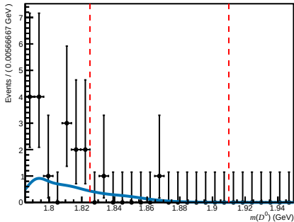
Passed ( 200 < n\text{Tracks} < 600 , 3.6 < \eta < 5.0 , 6000 < p < 10000 )
