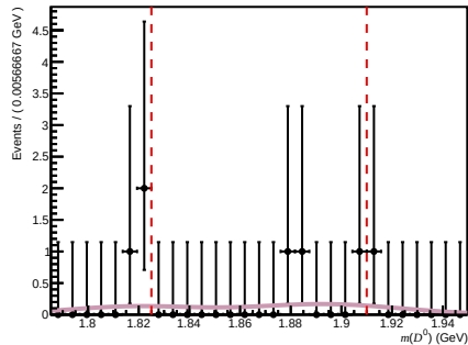
Total ( 200 < n\text{Tracks} < 600 , 3.6 < \eta < 5.0 , 10000 < p < 15600 )
