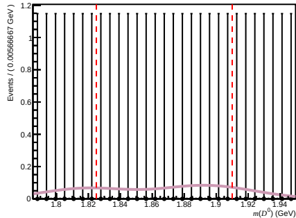
Passed ( 200 < n\text{Tracks} < 600 , 3.6 < \eta < 5.0 , 10000 < p < 15600 )
