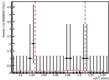
Failed ( 200 < n\text{Tracks} < 600 , 3.6 < \eta < 5.0 , 10000 < p < 15600 )
