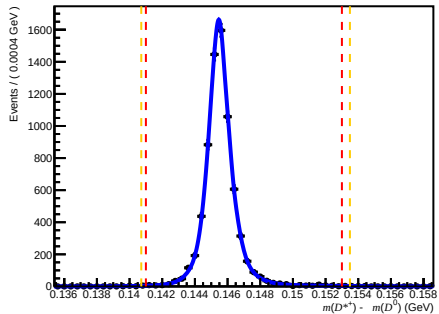
Passed DiF (after RICH1) ( 0 < nTracks < 200 , 1.7 < \eta < 3.6 , 3000 < p < 6000 )
