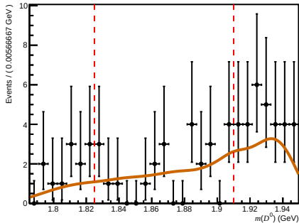
Passed ( 0 < n\text{Tracks} < 200 , 3.6 < \eta < 5.0 , 10000 < p < 15600 )
