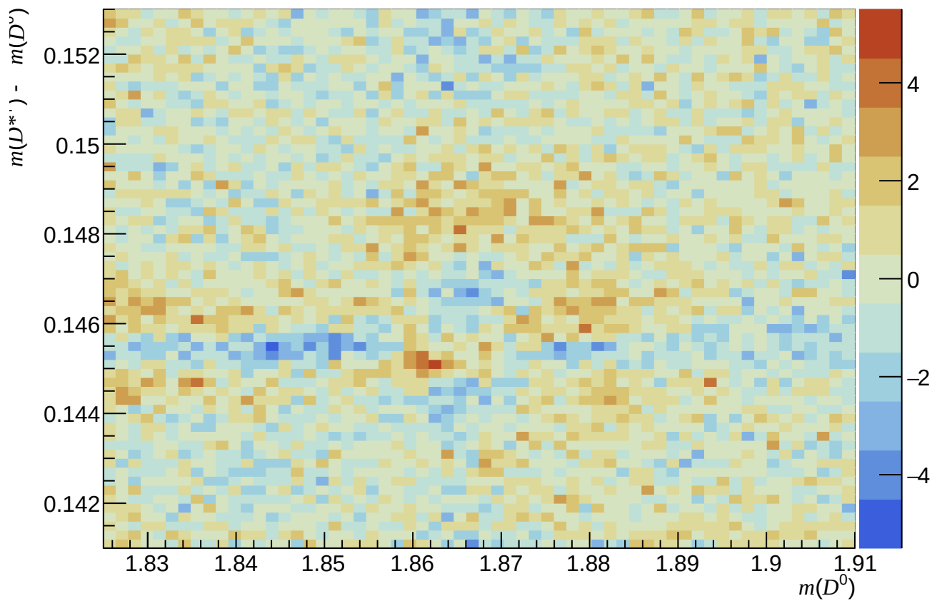
Failed ( 200 < n\text{Tracks} < 600 , 1.7 < \eta < 3.6 , 6000 < p < 10000 )
