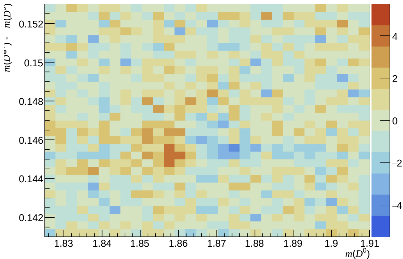
Passed ( 200 < n\text{Tracks} < 600 , 1.7 < \eta < 3.6 , 6000 < p < 10000 )
