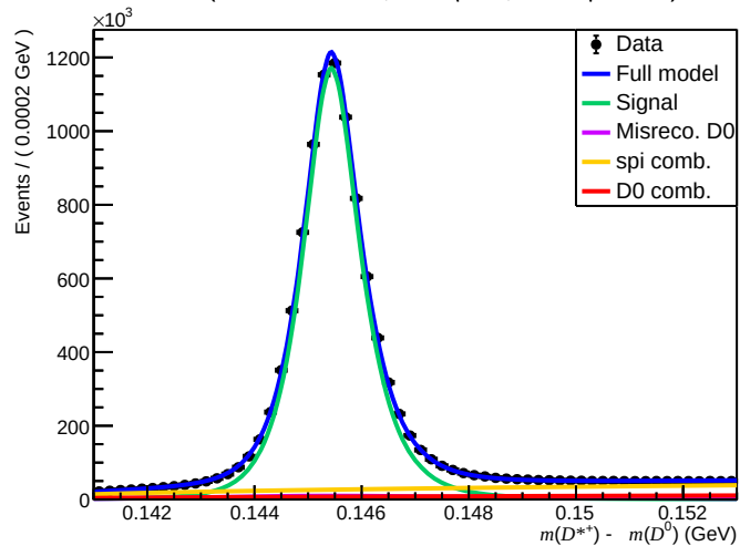
Failed (200 < nTracks < 600, 1.7 < \eta < 3.6, 15600 < p < 27000)
