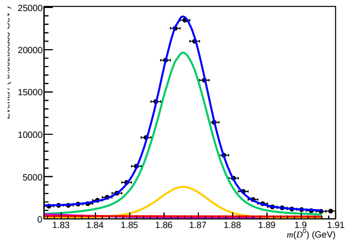
Failed (200 < nTracks < 600, 1.7 < \eta < 3.6, 15600 < p < 27000)
