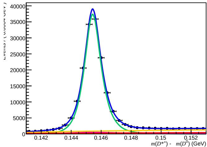
Failed (200 < nTracks < 600, 1.7 < \eta < 3.6, 15600 < p < 27000)
