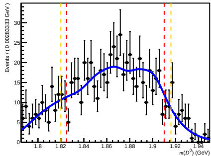
Passed DiF (after RICH1) ( 200 < nTracks < 600 , 1.7 < \eta < 3.6 , 60000 < p < 100000 )
