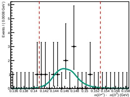
Passed ( 0 < n_{\text{Tracks}} < 200 , 3.6 < \eta < 5.0 , 3000 < p < 6000 )
