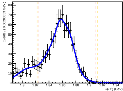
Passed DIF (after RICH1) ( 0 < n_{\text{Tracks}} < 200 , 3.6 < \eta < 5.0 , 6000 < p < 10000 )
