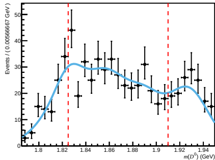
Total ( 0 < n_{\text{Tracks}} < 200 , 3.6 < \eta < 5.0 , 60000 < p < 100000 )
