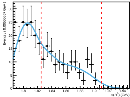
Failed ( 200 < nTracks < 600 , 1.7 < \eta < 3.6 , 3000 < p < 6000 )
