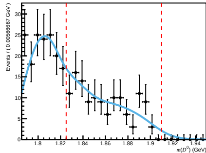
Total ( 200 < nTracks < 600 , 1.7 < \eta < 3.6 , 3000 < p < 6000 )
