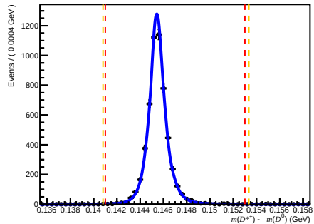
Passed Df (after RICH1) ( 200 < nTracks < 600 , 1.7 < \eta < 3.6 , 6000 < p < 10000 )
