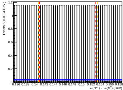
Passed Df (before RICH1) ( 200 < nTracks < 600 , 1.7 < \eta < 3.6 , 6000 < p < 10000 )
