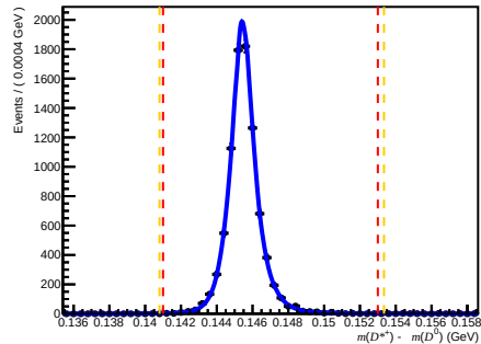
Failed Df ( 200 < nTracks < 600 , 1.7 < \eta < 3.6 , 6000 < p < 10000 )
