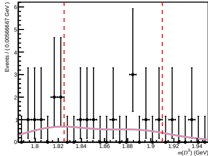
Total ( 200 < nTracks < 600 , 3.6 < \eta < 5.0 , 3000 < p < 6000 )
