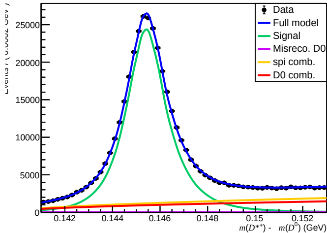
Failed ( 200 < n\text{Tracks} < 600 , 3.6 < \eta < 5.0 , 6000 < p < 10000 )
