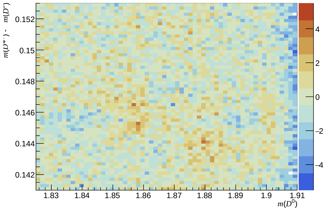
Failed ( 200 < n\text{Tracks} < 600 , 3.6 < \eta < 5.0 , 6000 < p < 10000 )
