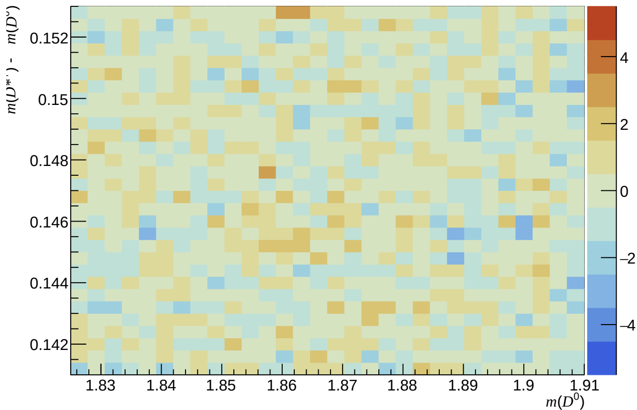
Passed ( 200 < n\text{Tracks} < 600 , 3.6 < \eta < 5.0 , 6000 < p < 10000 )
