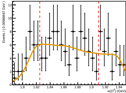
Passed ( 0 < n_{\text{Tracks}} < 200 , 3.6 < \eta < 5.0 , 6000 < p < 10000 )
