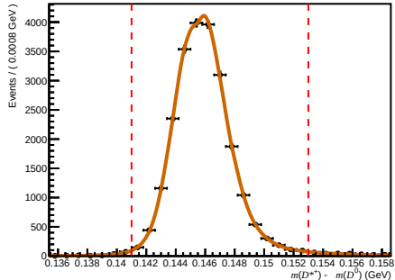
Failed ( 0 < n\text{Tracks} < 200 , 3.6 < \eta < 5.0 , 27000 < p < 60000 )
