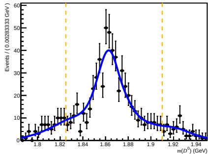
Passed DiF (after RICH1) ( 200 < nTracks < 600 , 1.7 < \eta < 3.6 , 10000 < p < 15600 )
