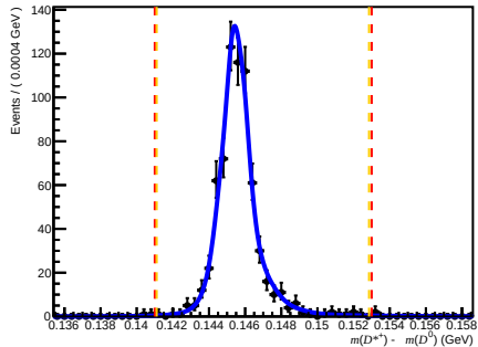
Passed DiF (after RICH1) ( 200 < n_{\text{Tracks}} < 600 , 1.7 < \eta < 3.6 , 10000 < p < 15600 )
