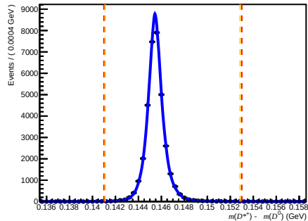
Failed DiF ( 200 < n_{\text{Tracks}} < 600 , 1.7 < \eta < 3.6 , 10000 < p < 15600 )
