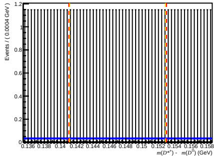
Passed DiF (before RICH1) ( 200 < n_{\text{Tracks}} < 600 , 1.7 < \eta < 3.6 , 10000 < p < 15600 )
