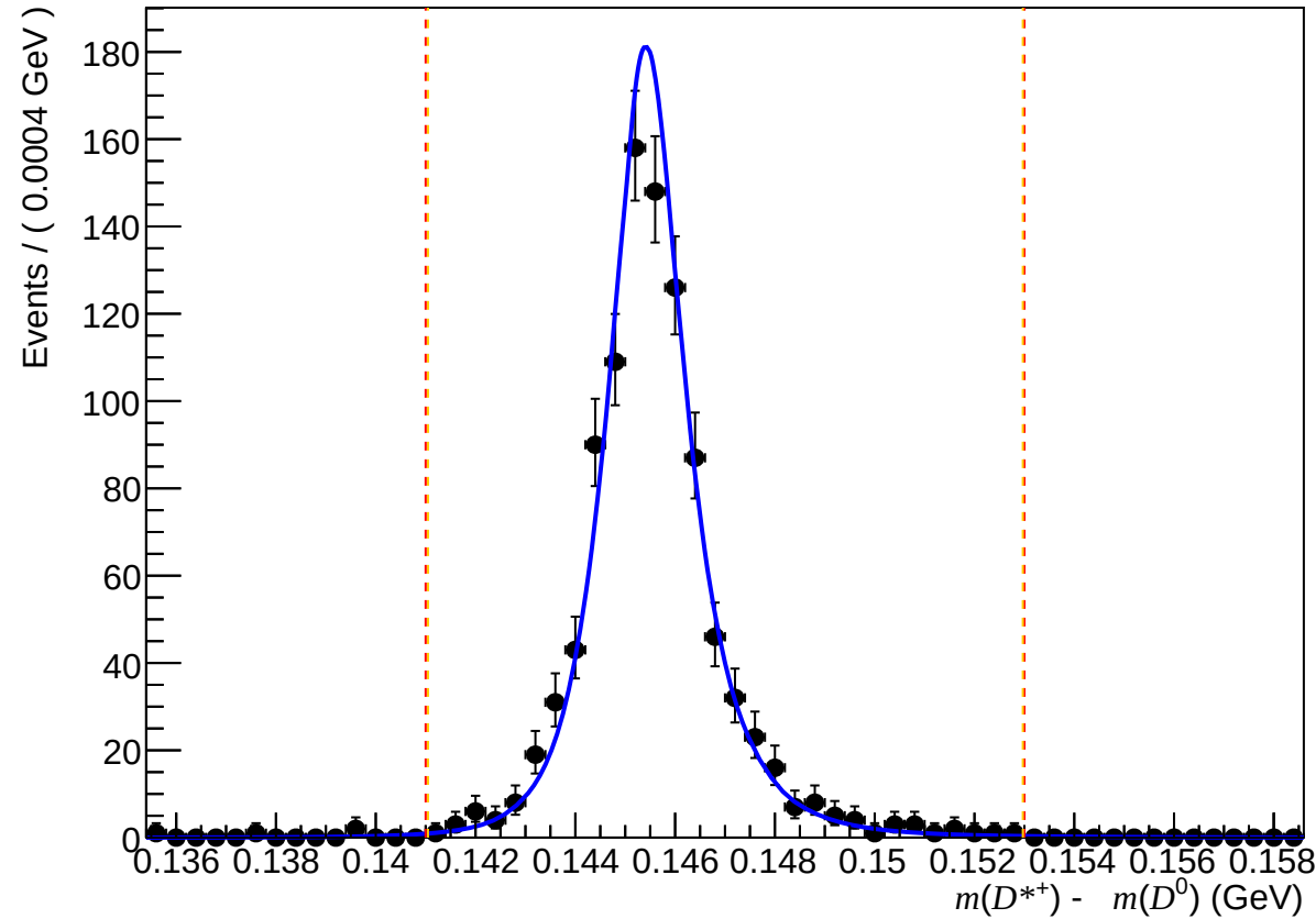
Passed non-DiF ( 200 < nTracks < 600 , 3.6 < \eta < 5.0 , 15600 < p < 27000 )
