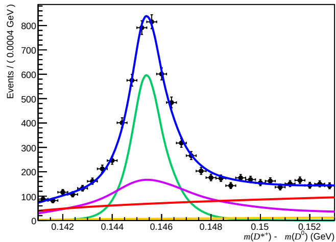
Failed ( 0 < n_{\text{Tracks}} < 200 , 1.7 < \eta < 3.6 , 60000 < p < 100000 )
