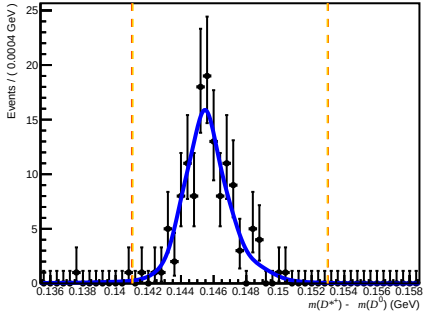
Passed DiF (before RICH1) ( 0 < nTracks < 200 , 3.6 < \eta < 5.0 , 3000 < p < 6000 )
