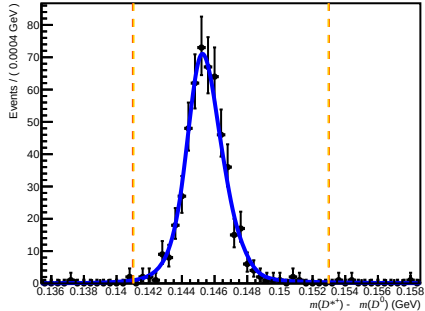
Passed DiF (after RICH1) ( 0 < nTracks < 200 , 3.6 < \eta < 5.0 , 3000 < p < 6000 )
