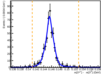
Failed DiF ( 0 < nTracks < 200 , 3.6 < \eta < 5.0 , 3000 < p < 6000 )
